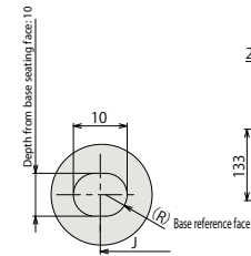
Detailed view Q Base elongated hole details
